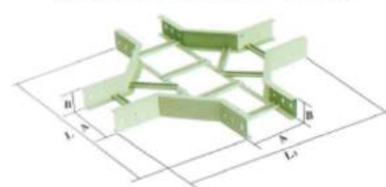
梯式水平等径四通XQJ-T1-04A
