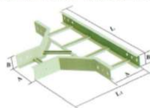
梯式水平等径三通XQJ-T1-03A
